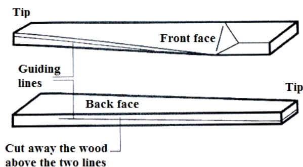
Fig 6: Twisted and tapered blade of correct thickness
