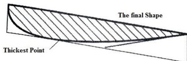
Fig 7: The finished cross section of the blade
