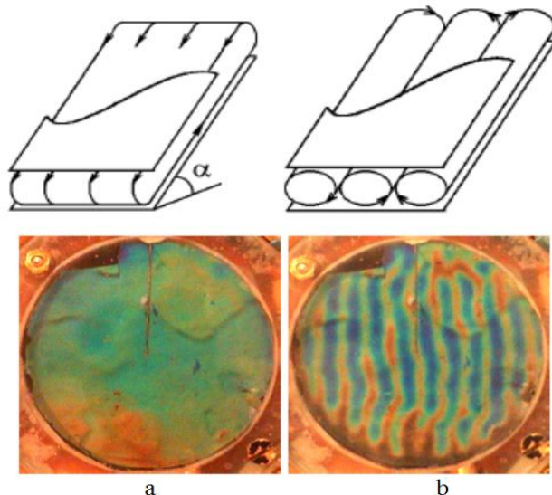
Fig. 2 Structures of convective motions and temperature distribution on a liquid crystal film in an inclined nanofluid layer heated from below: a – basic lifting – drop flow; b – the Rayleigh component. The photos were taken from the upper heat exchanger at \alpha = 10^\circ and \Delta T : (a) 8 K; (b) 16 K.
