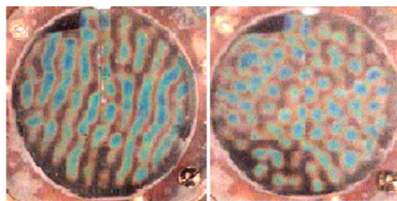
Fig. 4 Cross – roll instability of convective rolls at \alpha = 5^\circ , \Delta T/\Delta T_C = 1.4 ; the interval between shots is 6 minutes.
