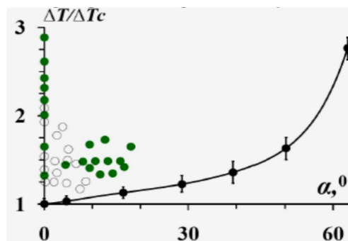
Fig. 3 A cross – roll region of instability in an inclined heated from below layer of nanofluid: dispersion dots – the stability boundary of a primary flow; colorless circles – target – formed and spiral convective rolls; solid circles – extended convective rolls.
