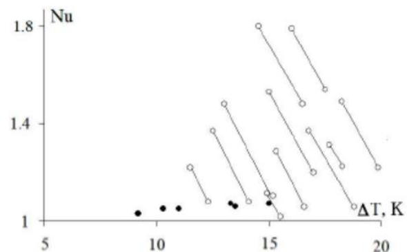
Fig. 11 Convective heat transfer in an inclined layer of nanofluid at \alpha = 15^\circ ; black dots are corresponded to the primary flow in the case of gradually increasing \Delta T .
