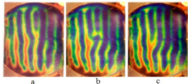
Fig. 10 Modulated convective rolls at \alpha = 15^\circ , \Delta T/\Delta T_C = 2.4 ; the time between shots is 1 min.
