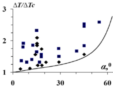
Fig 5. The area of amplitude modulation of the Rayleigh convection in an inclined heated from below layer of nanofluid: rhombuses –spontaneous decay and excitation of convection throughout the layer; squares – floating convective "spots".
