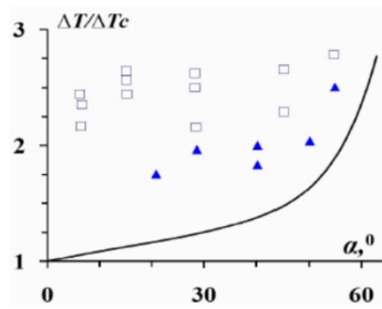
Fig. 8 Area of running convective rolls in an inclined heated from below layer of nanofluid: triangles – "flickering states"; squares – rolls with dislocations.
