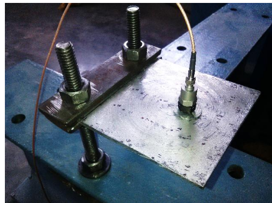
Fig.3 Plate fixed with CFFF condition
