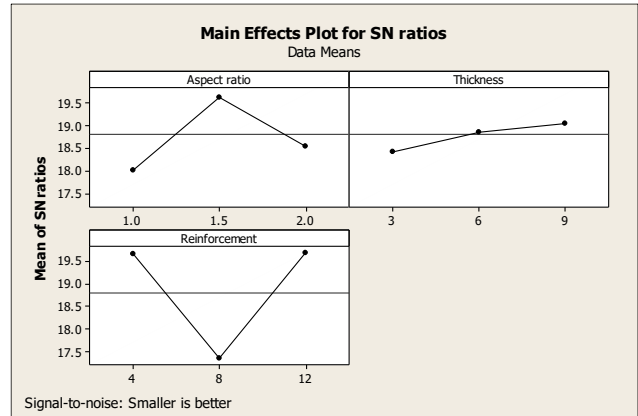
Fig.7 Main effect plot for SN ratios (smaller is better) CFCF
