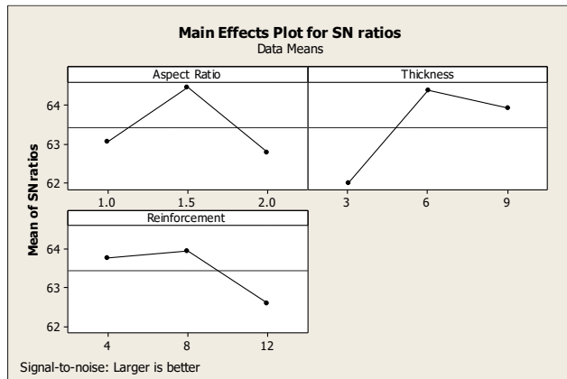
Fig.9 Main effect plot for SN ratios (larger is better) CFCF
