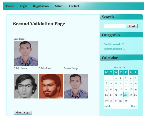
Fig.3: VCS Method
