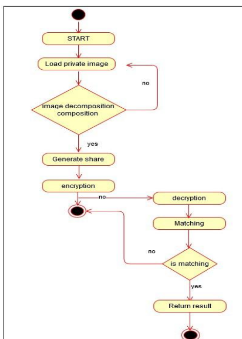
Fig.2: Activity diagram
