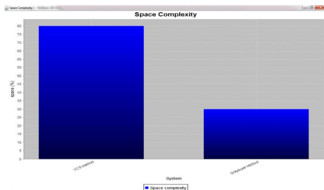
Fig.5: Space Complexity
