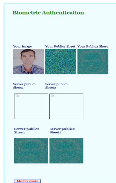
Fig.4: GEVCS Method
