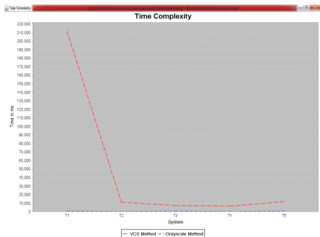
Fig.5: Time Complexity
