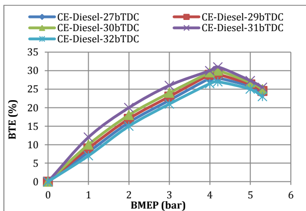
Fig.3 variation of brake thermal efficiency (BTE) with brake mean effective pressure (BMEP) in the conventional engine with neat diesel, at various injection timings at an injector opening pressure of 190 bar
