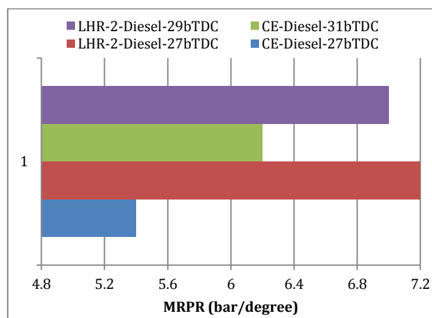
Fig.9 Bar charts showing the variation of maximum rate of pressure rise (MRPR) at full load with injection timing with both versions of the combustion chamber
