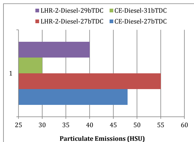
Fig.5 Bar charts showing the variation of particulate emissions at full load with injection timing with both versions of the combustion chamber
