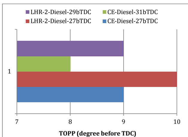
Fig.10 Bar charts showing the variation of time of occurrence of peak pressure (TOPP) at full load with injection timing with both versions of the combustion chamber
