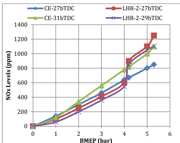
Fig.6 Variation of nitrogen oxide (NO x ) levels with brake mean effective pressure (BMEP) in conventional engine (CE) and engine with LHR-2 combustion chamber at recommended injection timing and at optimized injection timing at an injector opening pressure of 190 bar
