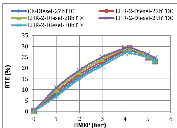
Fig.3 variation of brake thermal efficiency (BTE) with brake mean effective pressure (BMEP) in the engine with LHR-2 combustion chamber with neat diesel, at various injection timings at an injector opening pressure of 190 bar
