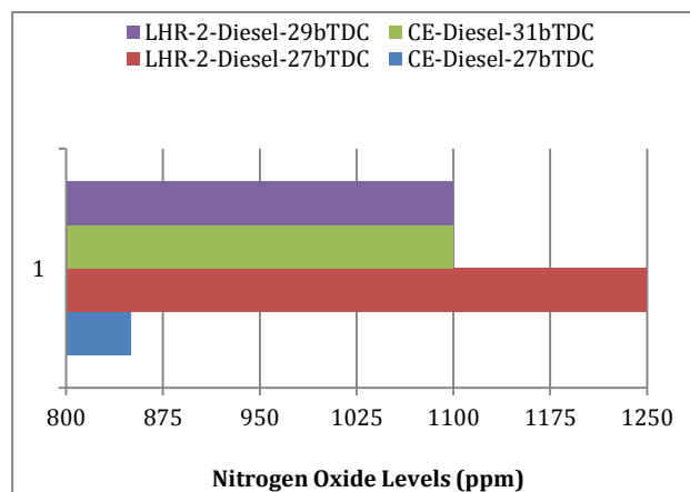
Fig.7 Bar charts showing the variation of nitrogen oxide levels (NO x ) at full load with injection timing with both versions of the combustion chamber
