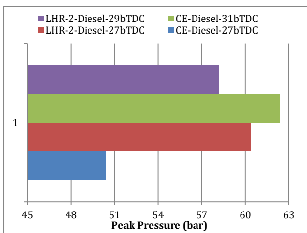
Fig.8 Bar charts showing the variation of peak pressure at full load with injection timing with both versions of the combustion chamber
