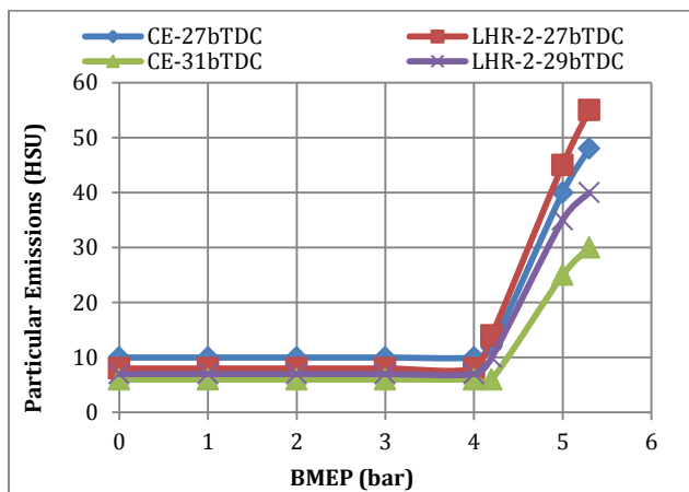
Fig.4 Variation of particulate emissions in Hartridge Smoke Unit (HSU) with brake mean effective pressure (BMEP) in conventional engine (CE) and engine with LHR-2 combustion chamber at recommended injection timing and at optimized injection timing at an injector opening pressure of 190 bar
