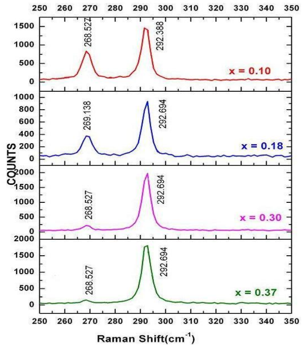
Fig.4 Raman spectrum for the samples
