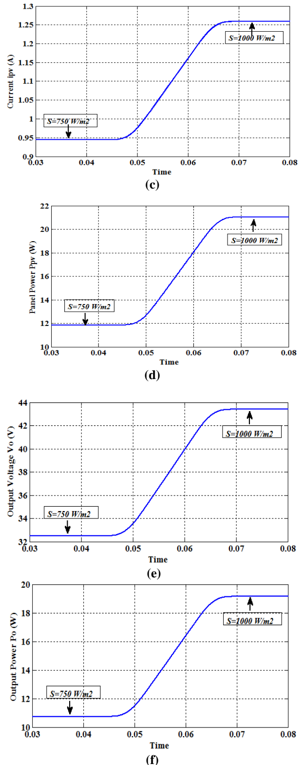
Fig. 9 Input-output characteristics at S_1=750 \text{ W/m}^2 to S_2=1000 \text{ W/m}^2 for boost converter and P&O controller (a) Panel voltage V_{pv} (b) Duty D (c) Inductor current I_{pv} (d) Input power P_{pv} (e) Output voltage V_o (f) Output power P_o
