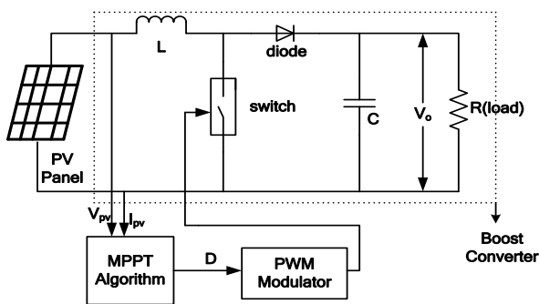
Fig.3 PV Panel along with Boost converter for MPP Tracking
