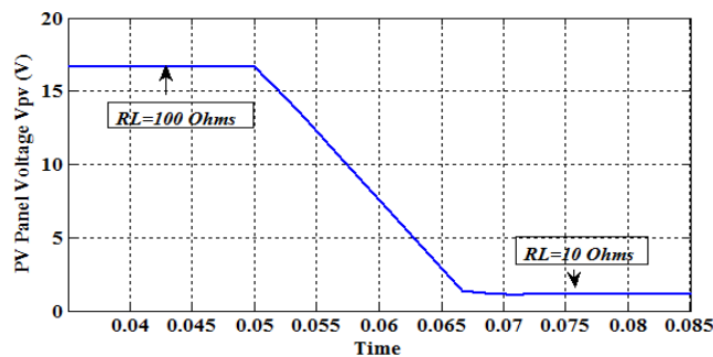
Fig.11 Operation of MPPT based on the boost converter in various load regions
