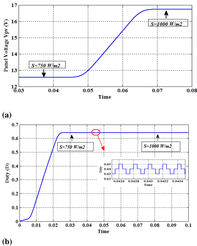
Fig. 9 Input-output characteristics at S_1=750 \text{ W/m}^2 to S_2=1000 \text{ W/m}^2 for boost converter and P&O controller (a) Panel voltage V_{pv} (b) Duty D (c) Inductor current I_{pv} (d) Input power P_{pv} (e) Output voltage V_o (f) Output power P_o
