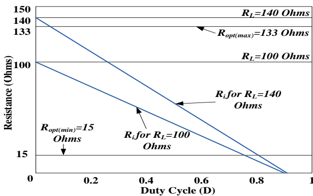
Fig.11 Operation of MPPT based on the boost converter in various load regions
