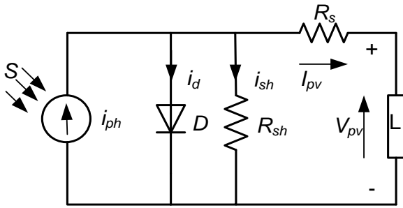
Fig.1 The equivalent circuit of Solar cell
